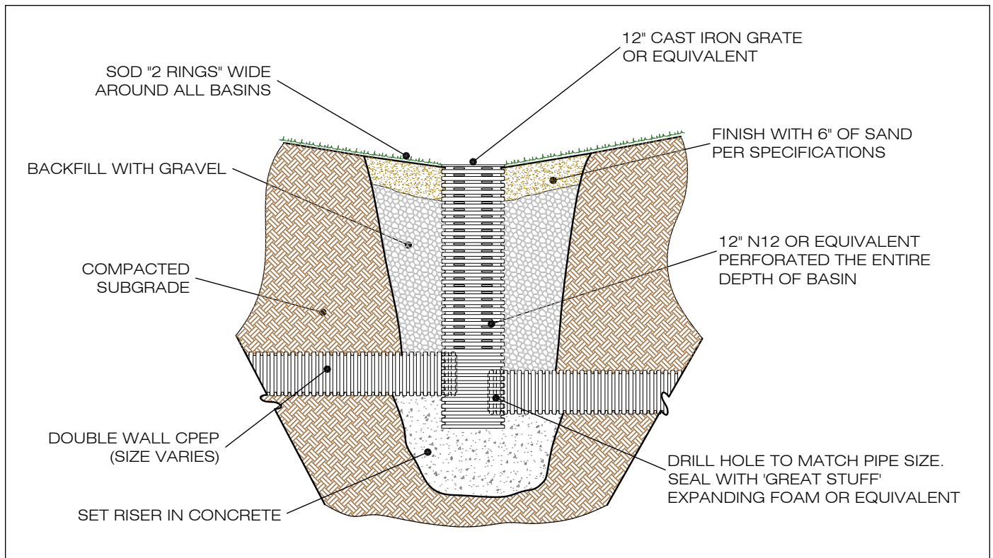
Figure 2-2. Typical catch basin design. Source: George Golf Design.
