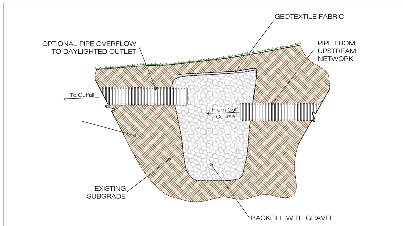
Figure 2-3. Drywell. Source: George Golf Design.
