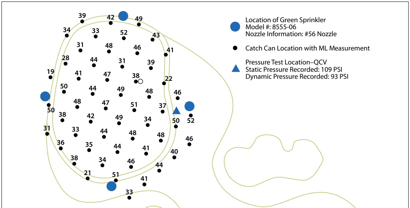
Figure D-3. Sample results of grid collection data, sprinkler information and pressures for green surface.
