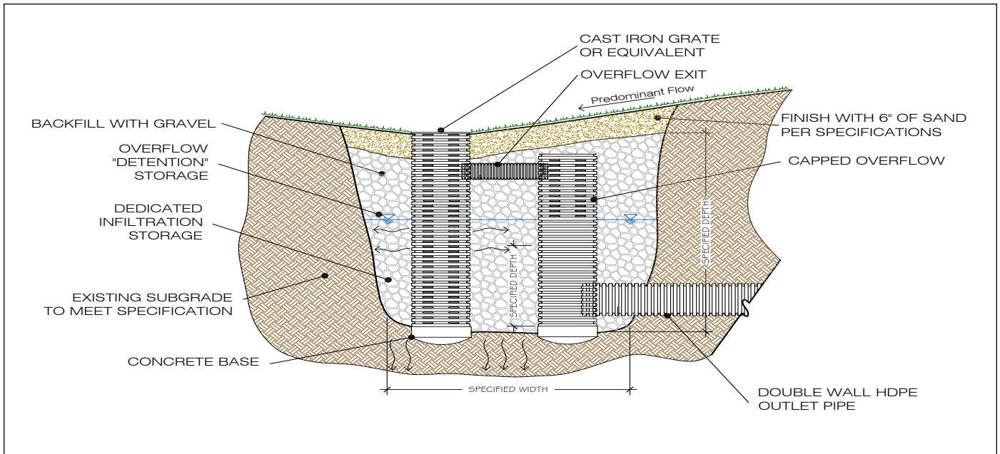
Figure 2-4. Modified infiltration catch basin. Source: George Golf Design.
