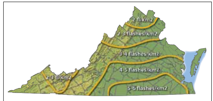
Figure 3-7. Lightning flash density map.
