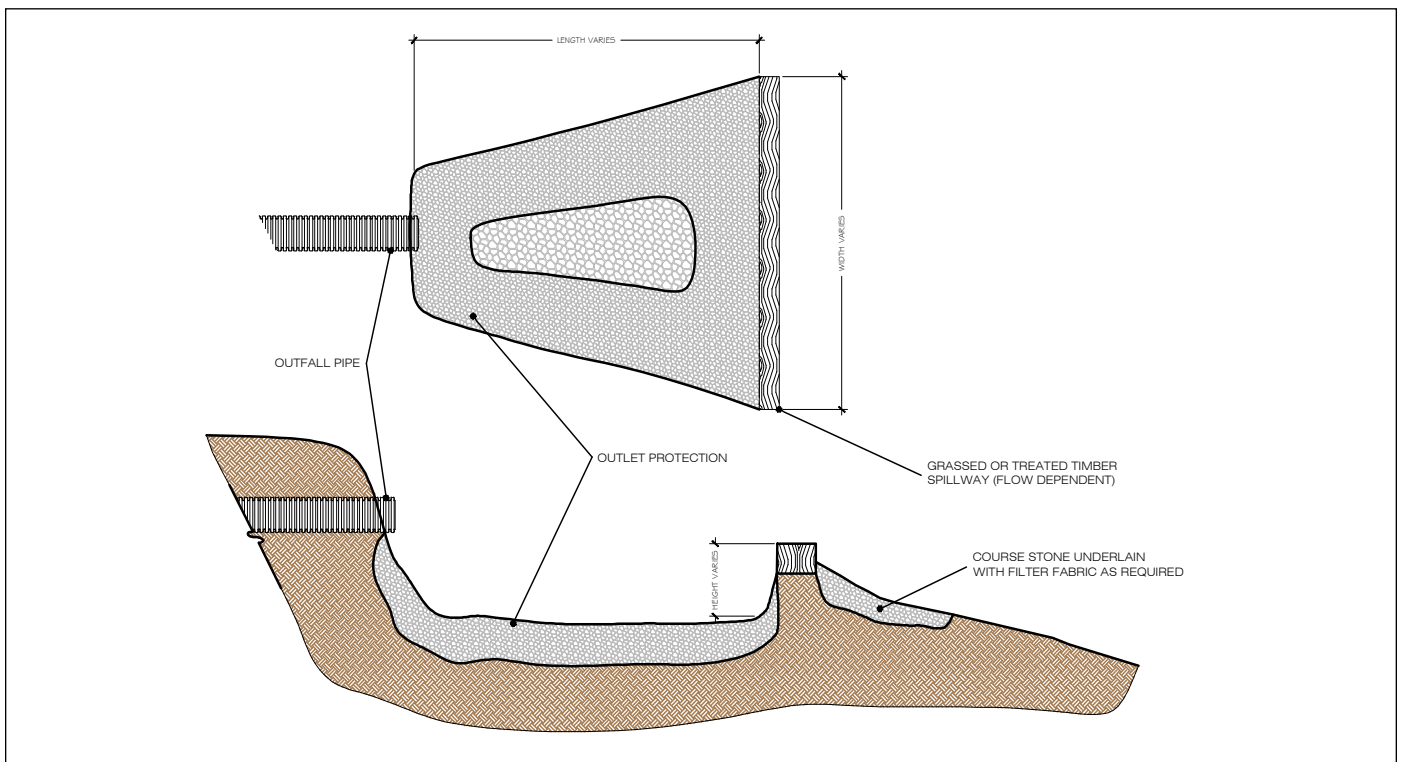
Figure 2-5. Level spreader. Source: George Golf Design.
