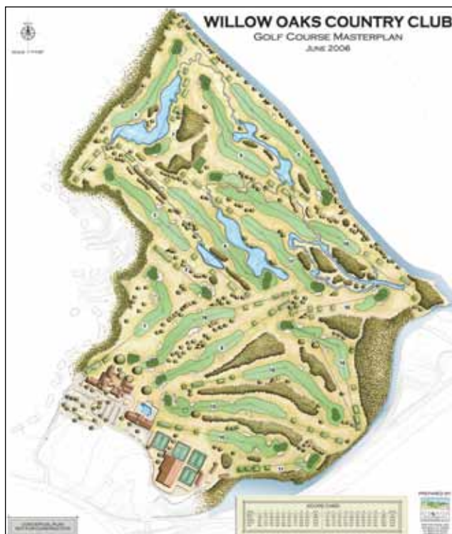
Figure B-1. Willow Oaks Country Club golf course redesign plan.
