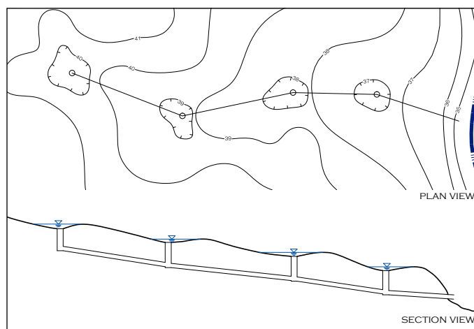
Figure 2-6. Soft draining swale used in combination with a small diameter pipe network. Source: George Golf Design.
